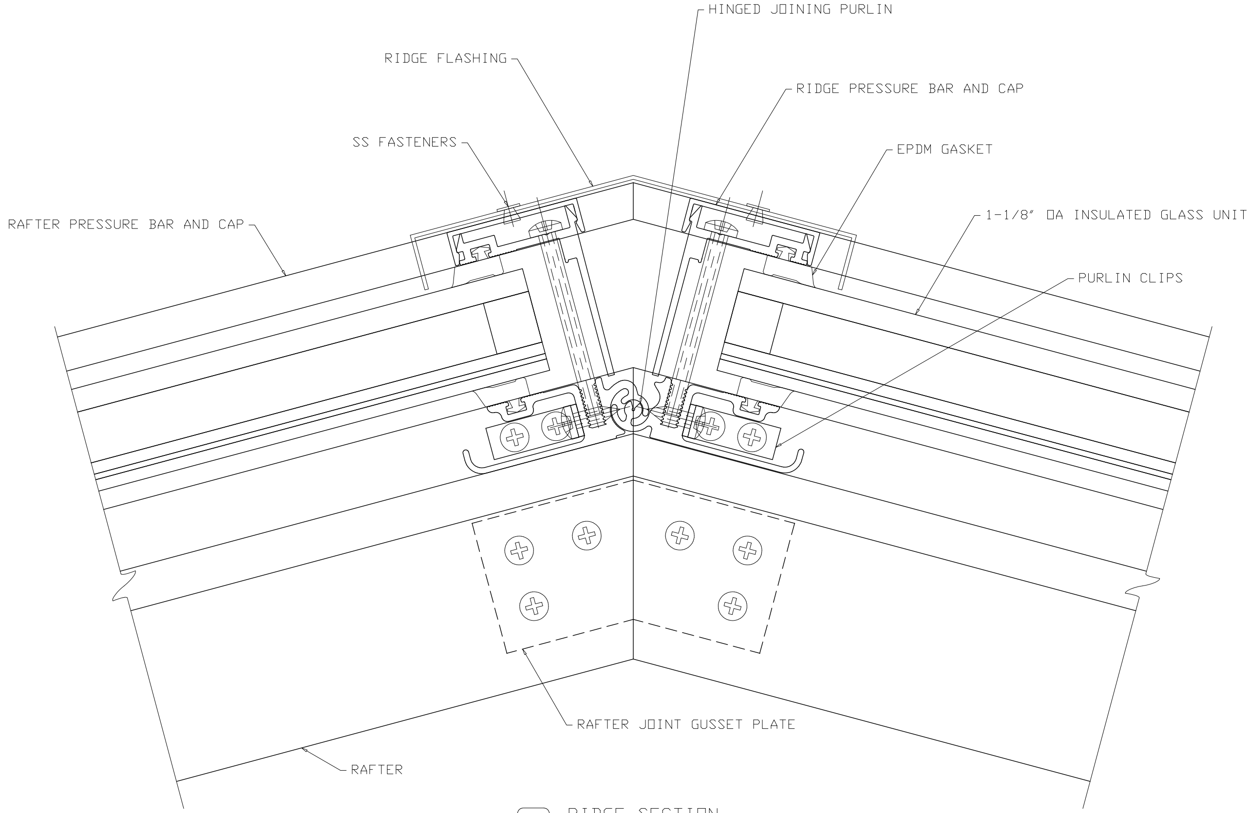
5 RIDGE SECTION SCALE 1' - 0" = 1' - 0"
