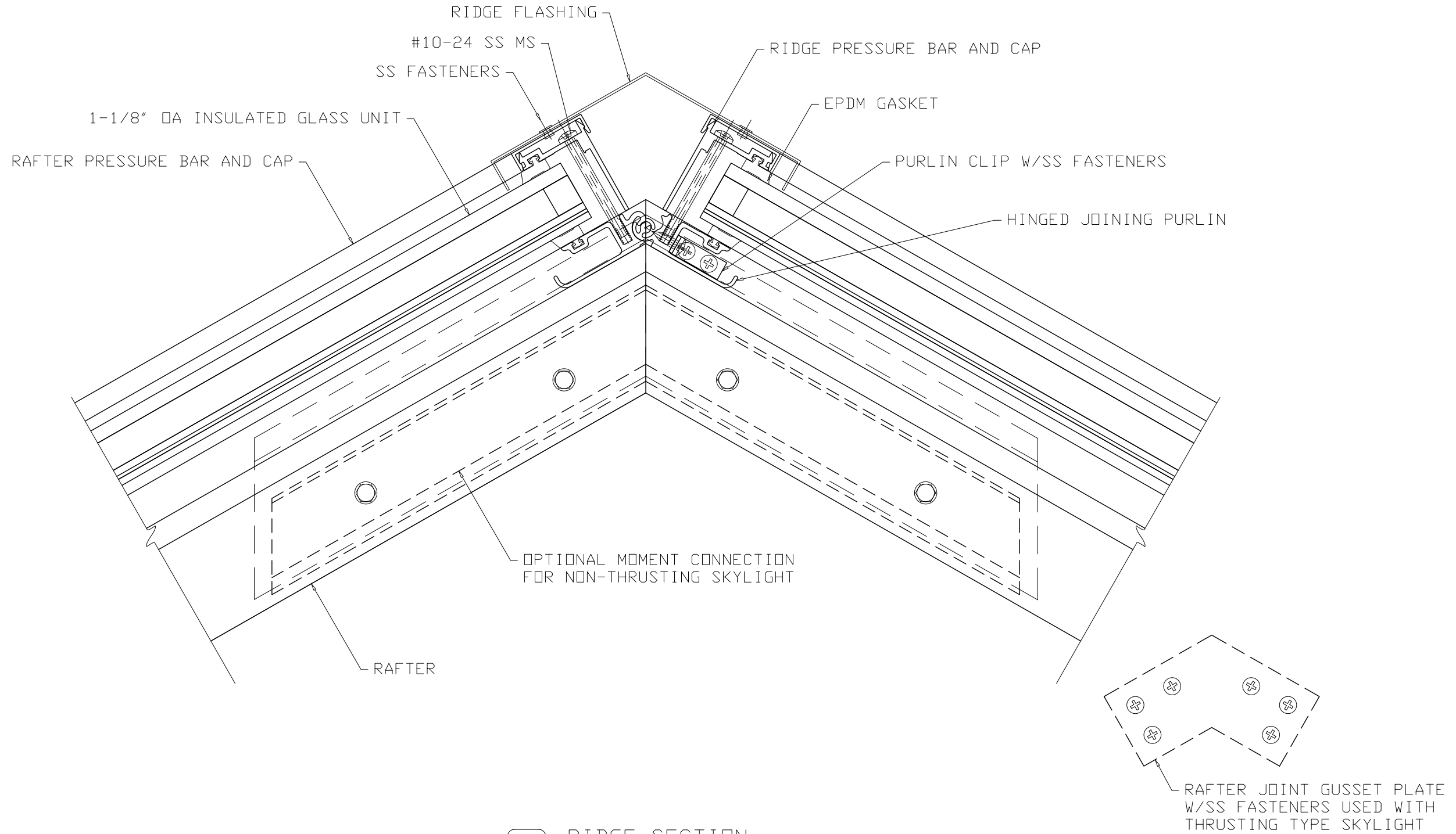
5 RIDGE SECTION SCALE 6"=1'-0"
