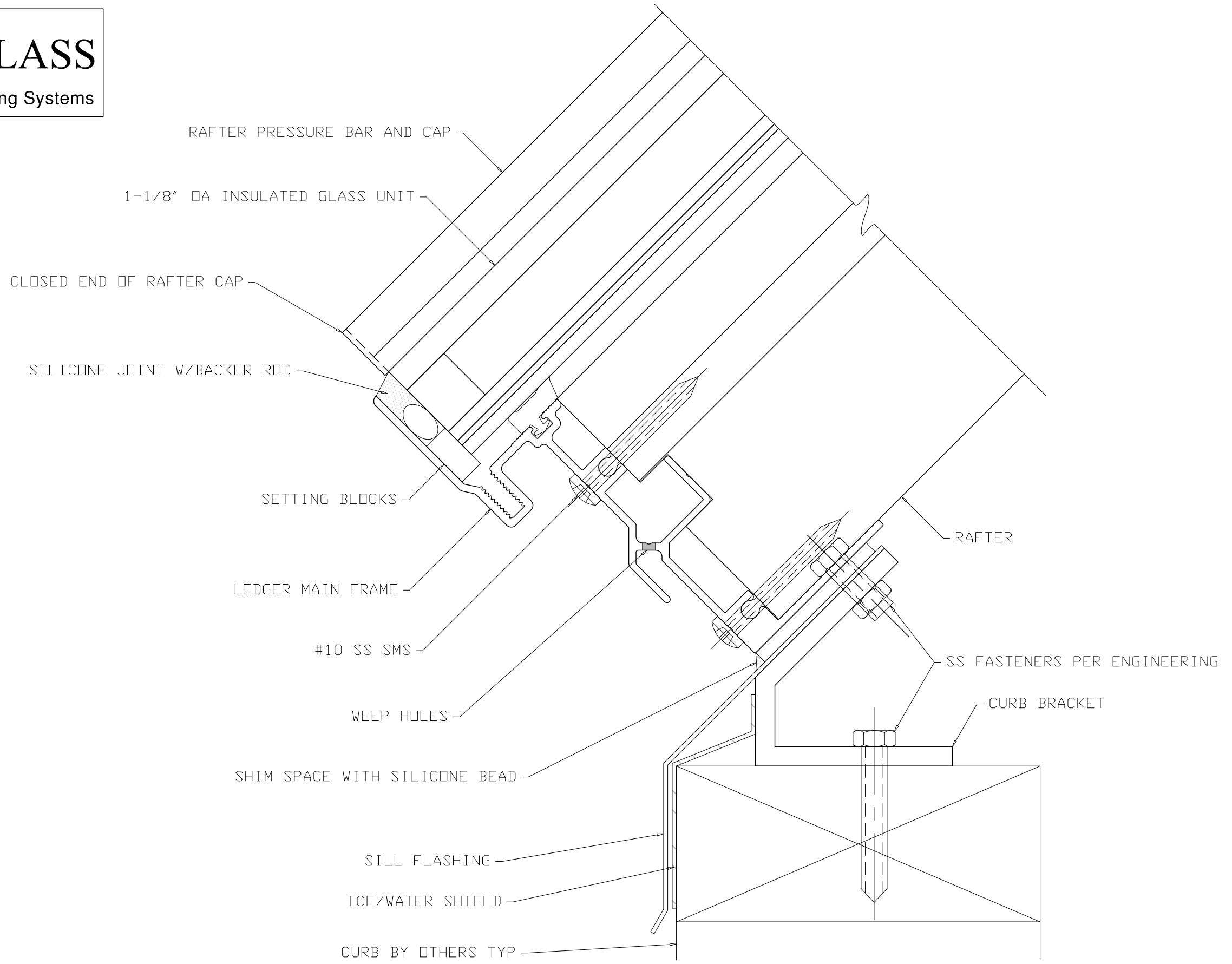
1 SILL SECTION SCALE 1' - 0" = 1' - 0"
